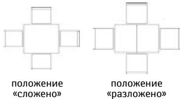
L800XB600XH750 L1200XB800XH750
